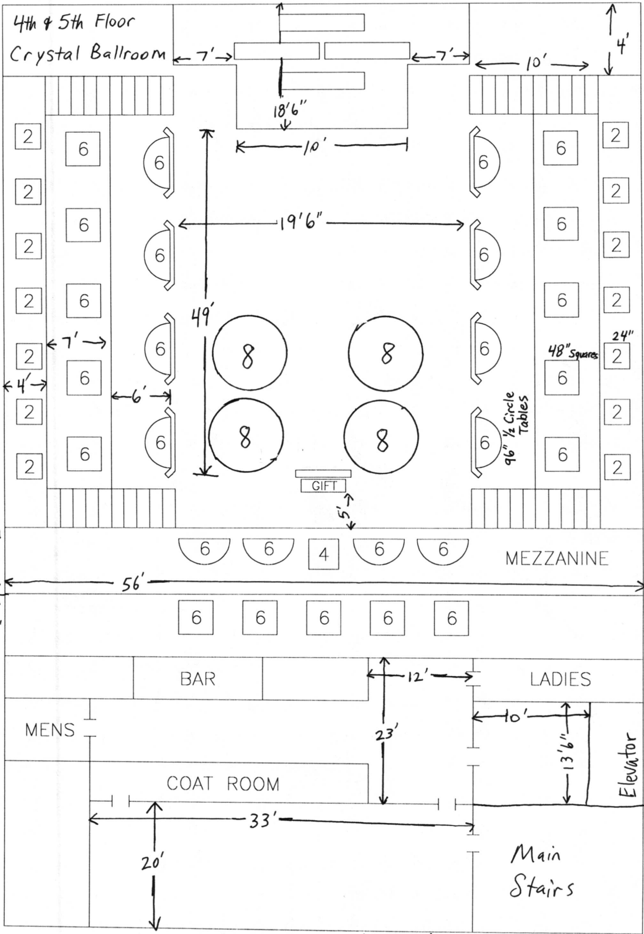
5th Floor App's Balcony 35'6" x 29'6"
